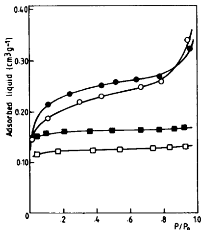
FIG. 3. Extent of the water (O) and n -hexane (□) adsorptions at 297 K on the Mo 793 sample. Filled symbols refer to the blank NaY zeolite.
