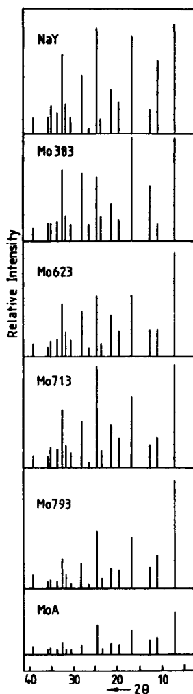
FIG. 1. X-ray powder diffraction patterns for NaY, Mo 383, Mo 623, Mo 713, Mo 793, and MoA samples.
