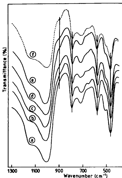
FIG. 2. Framework infrared spectra in the mid-wavenumber region for (a) NaY, (b) Mo 383, (c) Mo 623, (d) Mo 713, (e) Mo 793, and (f) MoA.
