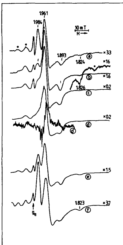
FIG. 7. ESR spectra of MoTe samples. (a) Sample Mo 623, outgassed 1 h at 573 K (measured at 295 K). For sample Mo 793E: (b) outgassed 2 h at 473 K; (c) subsequently outgassed (1 h) at 723 K; (d) heated 3 h under O_2 at 473 K (d', second derivative spectrum); (e) new sample portion outgassed 2 h at 393 K, then 1 h at 573 K; (f) subsequently heated under 3.7 \text{ kN m}^{-2} propylene (1 h) at 423 K. Spectra b-d measured at 77 K, spectra e-f measured at 295 K. Peaks marked with asterisk are due to hyperfine satellites arising from isotopes ^{95}\text{Mo} and ^{97}\text{Mo} (25% natural abundance).
