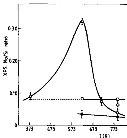
Fig. 5. Effect of the calcination temperature and procedure on the Mo/Si ratios of the samples as given by chemical analysis ( \square ) and by XPS: ( \circ ), MoT series, ( \bullet ) MoTE series, and ( \diamond ), MoA sample. Bars indicate estimated error.
