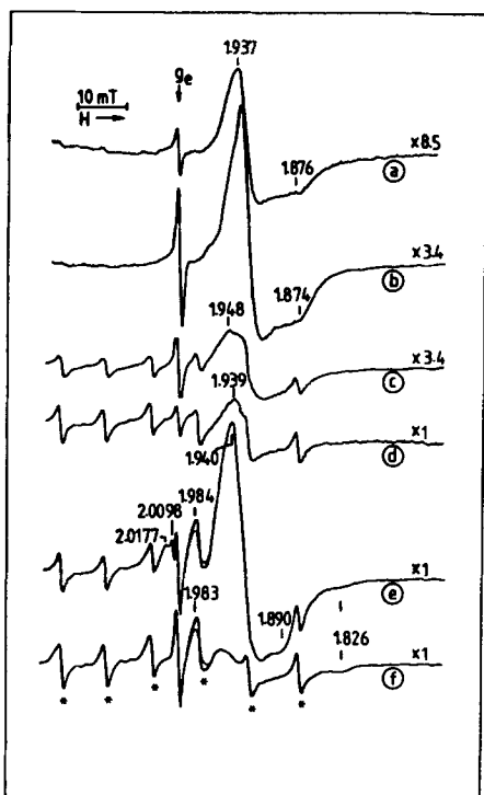
FIG. 6. ESR spectra of MoT samples. For sample Mo 623 (measured at 295 K): (a) outgassed 0.5 h at 373 K, then 1 h at 473 K; (b) after further outgassing (1 h) at 603 K; (c) after further outgassing (1 h) at 793 K. For sample Mo 793 (measured at 77 K): (d) outgassed 1 h at 373 K and 1 h at 473 K; (e) subsequently outgassed 1 h at 573 K; (f) heated overnight under O_2 at 523 K, then outgassed at 295 K. Sharp peaks marked with asterisk are due to Mn^{2+} impurity. The dashed line in spectra e and f marks the g_{\perp} peak of signal D, overlapping one of the Mn^{2+} lines.
