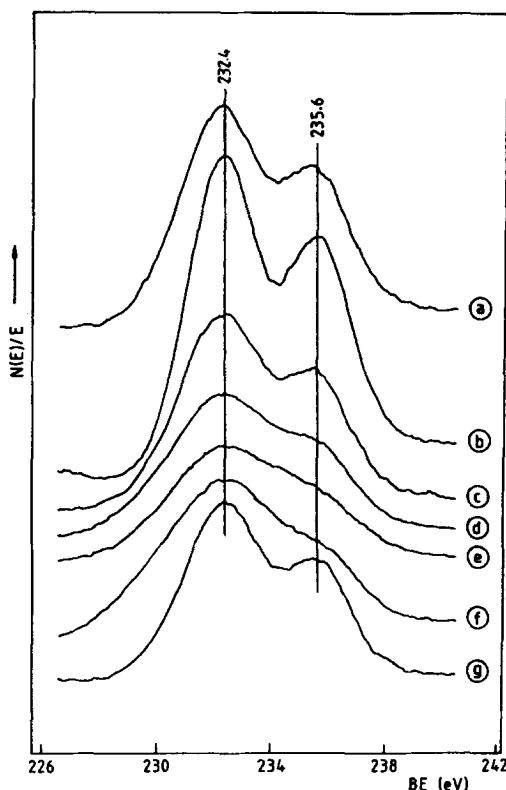
FIG. 4. Detailed XP spectra for molybdenum on different Mo-loaded NaY preparations: (a) Mo 383, (b) Mo 623, (c) Mo 713, (d) Mo 793, (e) Mo 623E, (f) Mo 793E, K and (g) MoA.
