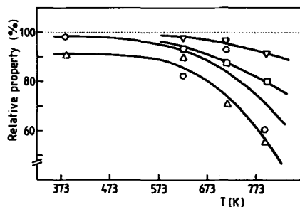
FIG. 8. Variation of crystallinity ( \circ ) and specific area ( \Delta ) with respect to the \text{MoO}_3\text{:NaY} physical mixture, and n -hexane ( \square ) and water ( \nabla ) sorption capacities with respect to NaY zeolite, as a function of the calcination temperature of the MoT series.
